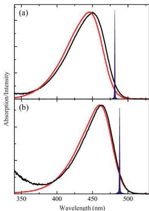
FIGURE 1 Ground state absorption spectrum of wild-type PYP ( a ) and the E-46Q mutant ( b ) in (dilute) solution (red lines) and in a crystalline lattice (black lines). The blue peak depicts the laser excitation spectrum for the crystalline samples. The spectra of the crystalline samples were measured with a polarized probe beam having the polarization plane oriented perpendicularly to the long axis of the crystal.
